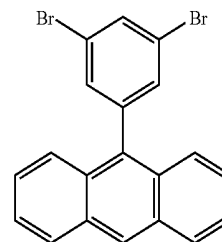
Intermediate Product 11-1
