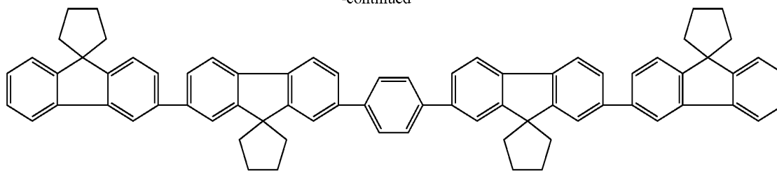
Compound (A61)
