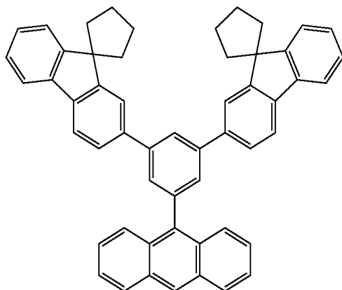
Intermediate Product 11-4
