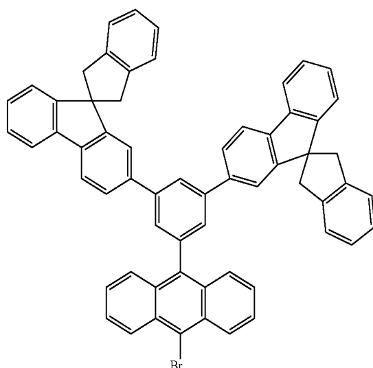
Intermediate Product 12-4
