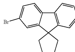
Intermediate Product 11-2
