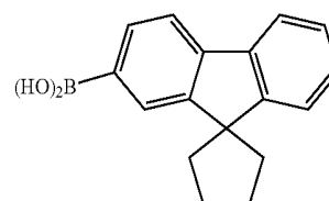
Intermediate Product 11-3
