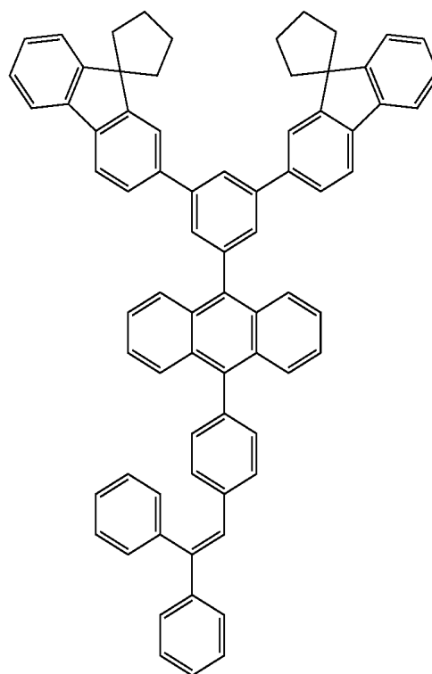
Compound (A11)
