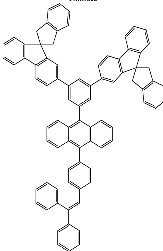
Compound (A12)
