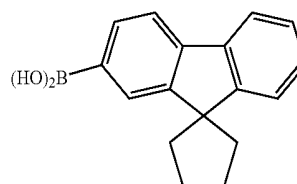
Intermediate Product 11-3
