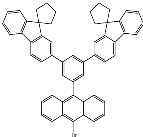
Intermediate Product 11-5
